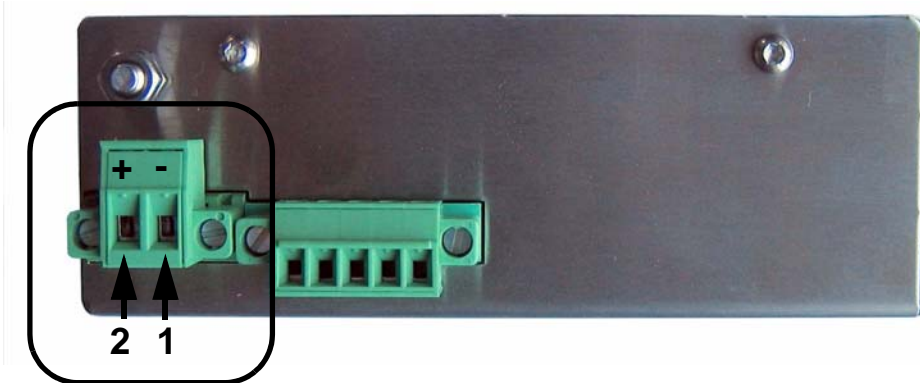
Figure 9: Power supply connector: eWON Mating female connector (included)
